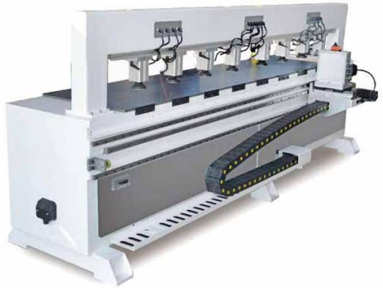
Multi Heads Wooden Door Lock CNC Hole Drilling Machine
